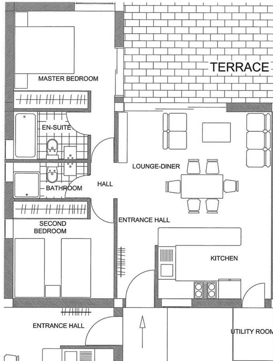
FIRST FLOOR APARTMENT B
